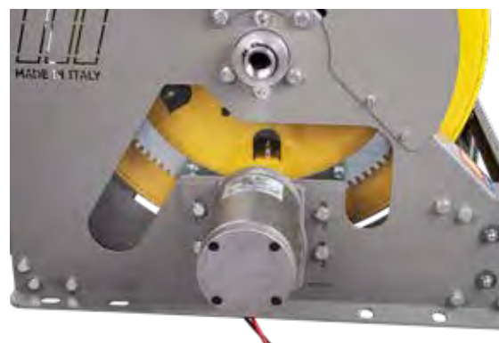
Direct motorized transmission with pinion on the sprocket
